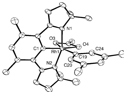
Figure 1. Molecular structure of 3 with ellipsoids at the 40% probability level (one of the molecules in the unit cell has been omitted for clarity). Selected bond lengths [Å] and angles [°]: Rh(1)–C(1) 1.919(2), Rh(1)–C(19) 1.993(2), Rh(1)–O(3) 2.2687(16), Rh(1)–O(4) 2.2673(16), Rh(1)–N(1) 2.0753(18), Rh(1)–N(2) 2.0580(18); N(2)–Rh(1)–N(1) 158.72(7), C(20)–C(19)–Rh(1) 128.83(17), C(24)–C(19)–Rh(1) 113.55(17).
