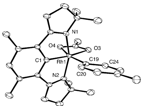
Figure 2. Molecular structure of 5p with ellipsoids at the 40% probability level (one of the molecules in the unit cell has been omitted for clarity). Selected bond lengths [Å] and angles [°]: Rh(1)–C(1) 1.912(2), Rh(1)–C(19) 2.005(2), Rh(1)–O(3) 2.2843(17), Rh(1)–O(4) 2.2328(18), Rh(1)–N(1) 2.0526(19), Rh(1)–N(2) 2.0592(19); N(1)–Rh(1)–N(2) 159.00(8), C(20)–C(19)–Rh(1) 128.69(19), C(24)–C(19)–Rh(1) 113.81(19).
